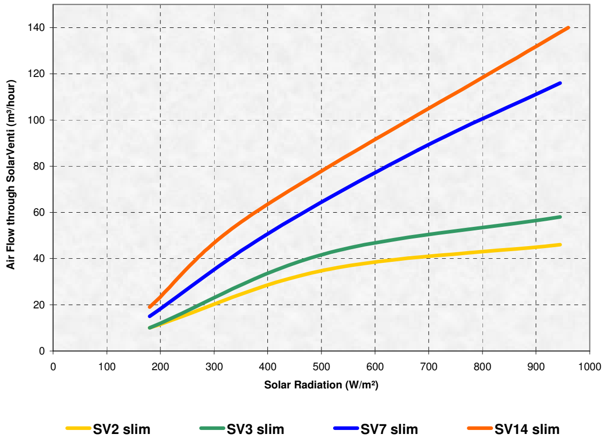
Air Flow / Solar Radiation for the New Slimline Models
